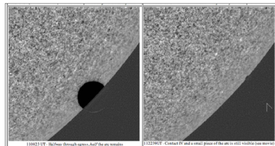
Figure 10: The atmosphere of Venus, at egress from TRACE (left), and (right) the last bit of Venus's silhouette on the solar disk (after Pasachoff, Schneider, and Widemann, 2011; courtesy: Lockheed Martin Solar and Astrophysics Laboratory and NASA).
