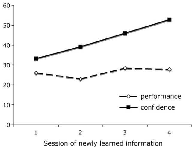
Fig. 1. A demonstration of increasing overconfidence: performance and confidence for each of the four sessions of newly learned and tested material. Figure created from the Oskamp's (1965) data.
