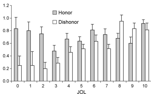
Fig. 2. Final test performance for the honor and dishonor conditions as a function of JOL.
