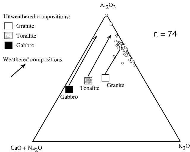
Fig. 5. Itremo Group pelite analyses shown on a major elements molar proportions plot. The diagram is modified after Nesbitt & Young (1984): total Ca is plotted because none of the samples was calcareous. Values for average gabbro, tonalite and granite are from Nesbitt & Young (1984). Pelite analyses are from this study (Table 2) and from Moine (1974).
